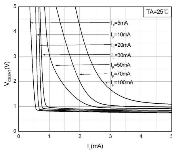
Fig.8 Collector-emitter Saturation Voltage vs. Forward Current
